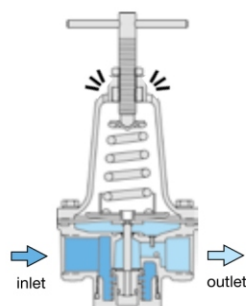
cross-section
