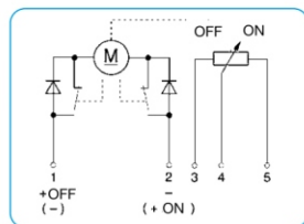
① DC motor w/ potentiometer 15
