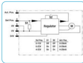
② with position controller 51
