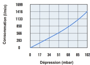
CDF 1500H-EPT200
