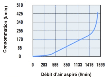
CDF 500H
