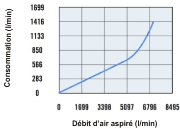
CDF 1500H
