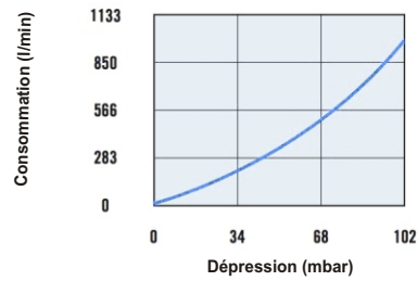
CDF 1000H-EPT125
