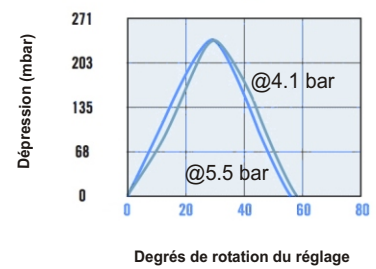
CDF 500H-EPT100-ST16FC
