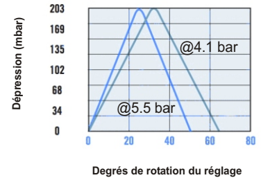
CDF 375H-EPT38-ST6BX
