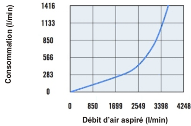
CDF 1000H
