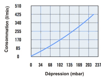
CDF 500H-EPT100
