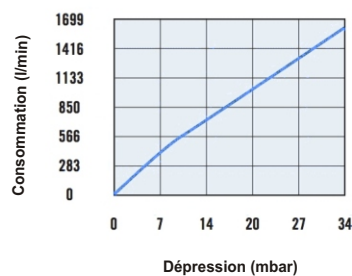
CDF 2000H
