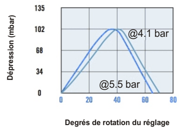
CDF 1500H-ST2020
