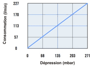
CDF 375H-EPT38
