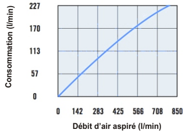
CDF 375H
