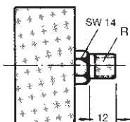
MA, round pressure gauge
