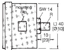
MB, square pressure gauge
