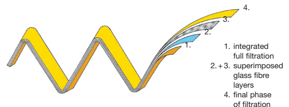
Cross-section showing complex construction of micro-filter elements
